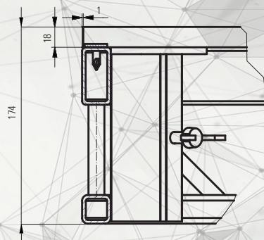
Cross section of profile
