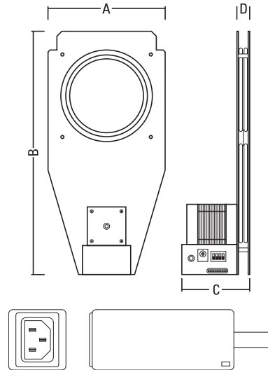
Separate PSU supplied with unit
